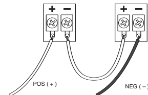
Figure 2. Series connection
