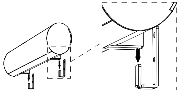
Slide Slots in Soundbar Feet onto Tabs on Brackets
